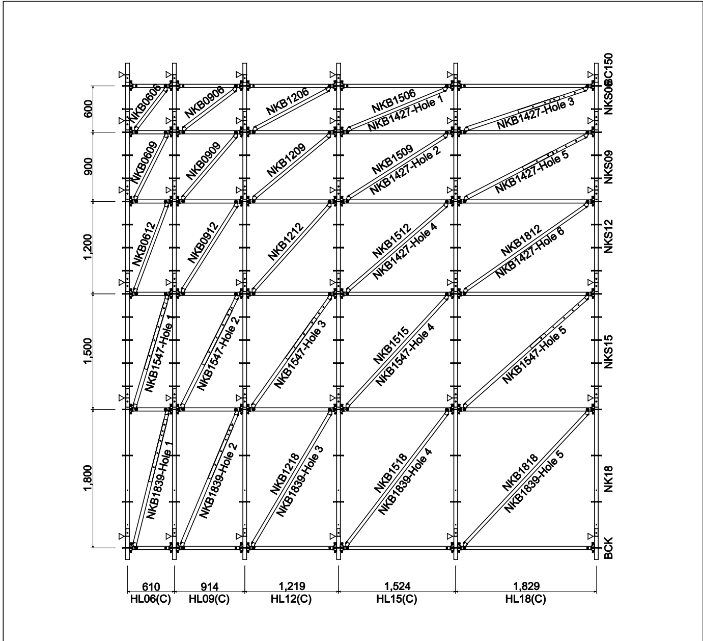
Example of arranging braces
