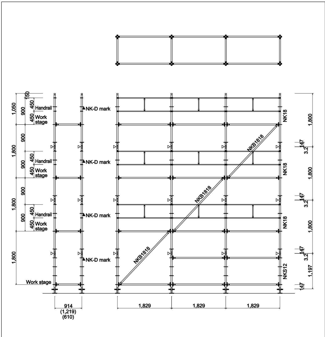
Example of arranging preceding handrail for scaffold
